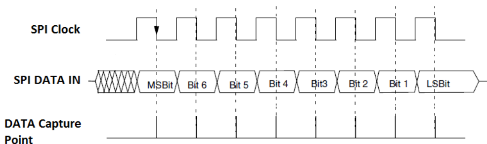
Figure 9: SPI input timing diagram
