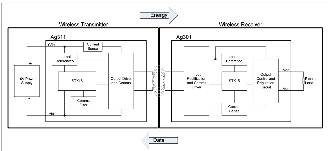
Figure 3: Charger Overview
