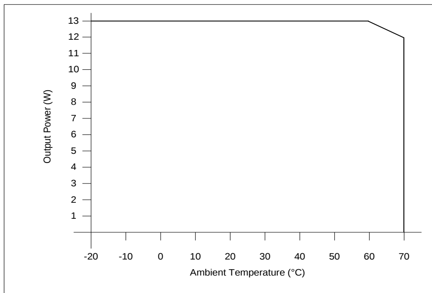
Figure 10: Ag9205 Operating Profile
