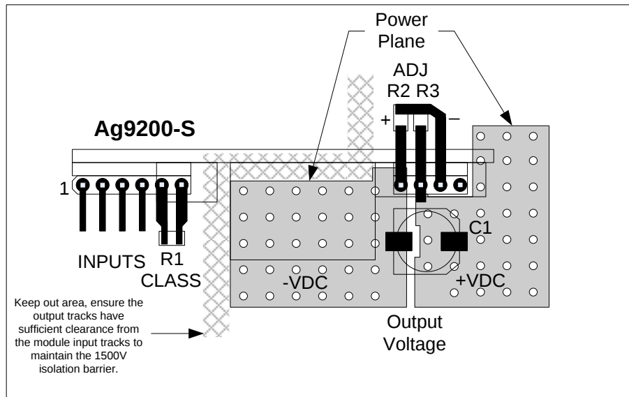
Figure 9: Power Plane Heatsink for Ag9200
